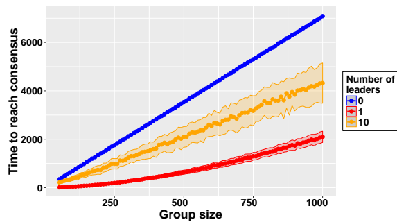
Figure 1: Time to reach consensus as a function of the size of the group for three different types of social organisation: (i) 0 leaders, (ii) 1 leader and (iii) 10 leaders. 100 independent replicates have been realised for each group size and social organisation. The ribbons represents the standard deviation across replicates.
